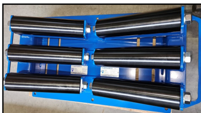
Execution with total 6 rollers for LENGTH rolling of pipe. Extra load capacity due to the 2 x 3 rollers. Model WRB-E-4-48-HD
